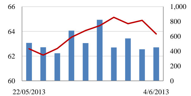
HNX- Index
